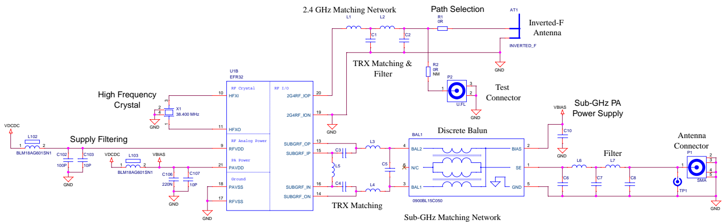
Figure 4.1. Schematic of the RF Section of the BRD4250B
